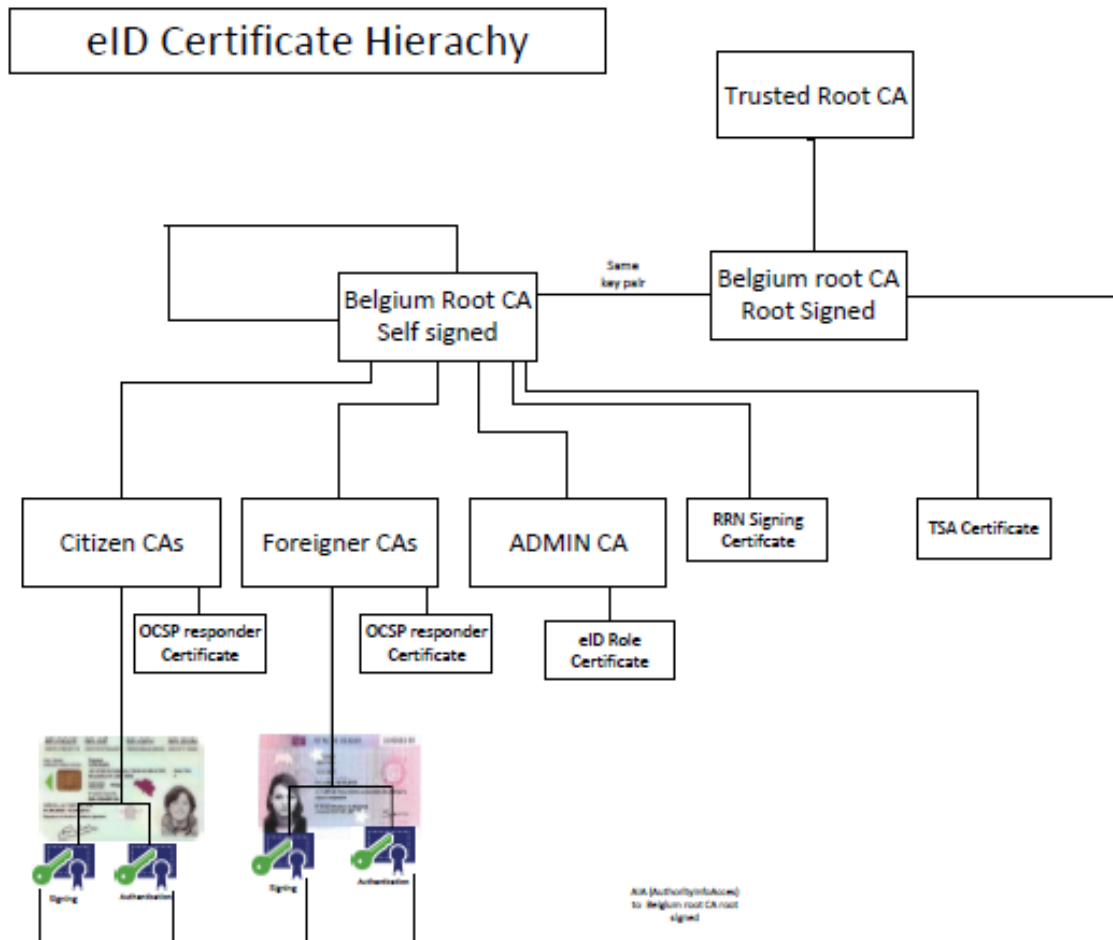
□ Figure 1: PKI hierarchy
